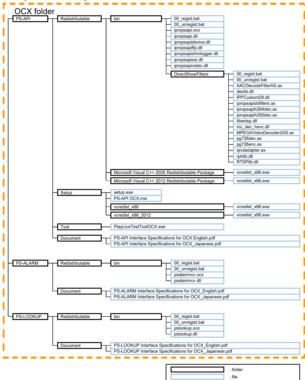
Figure 3-2 The layout of OCX directory
